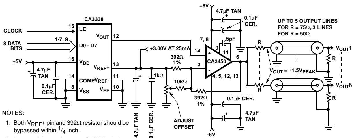
FIGURE 5. CA3338 DYNAMIC TEST CIRCUIT
