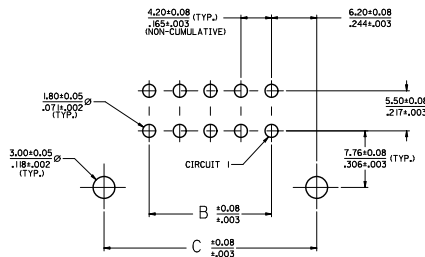
PCB LAYOUT, COMPONENT SIDE RECOMMENDED PCB THICKNESS: .160±0.18 .063±.007
