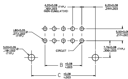
HEADER ASSEMBLY WITH NO CLIP OPTION
