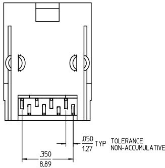
RECOMMENDED PANEL OPENING
