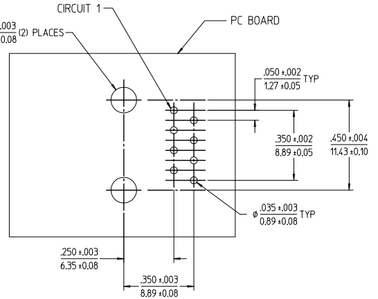
PCB LAYOUT: COMPONENT SIDE RECOMMENDED PCB THICKNESS: .062/1.57
