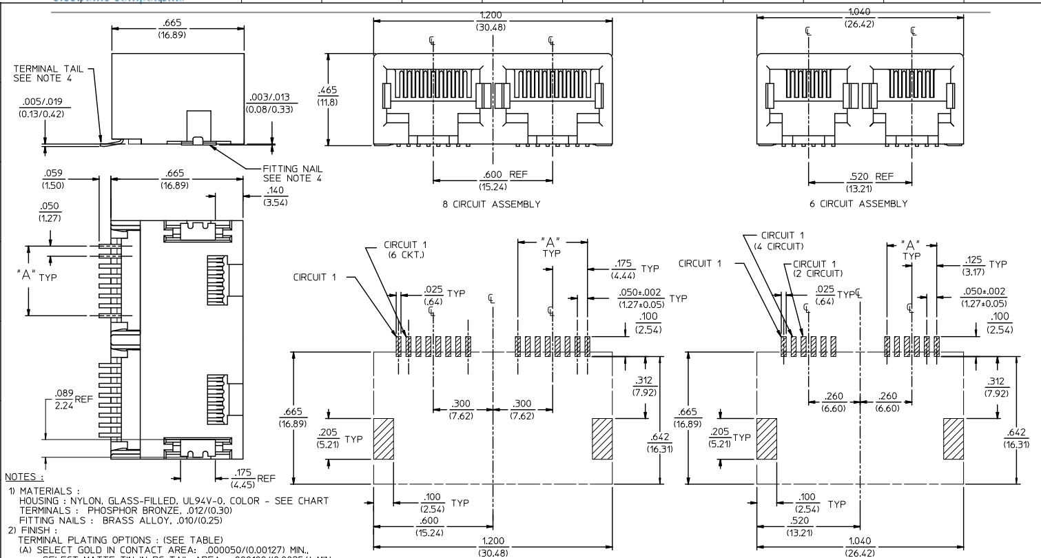
PC BOARD LAYOUT FOR 8 POSITION HOUSING
