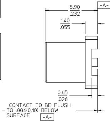
73415-1696 4 SLOT CONTACT
