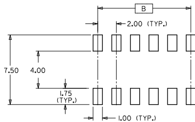
RECOMMENDED SOLDER PAD DESIGN (NTS)
