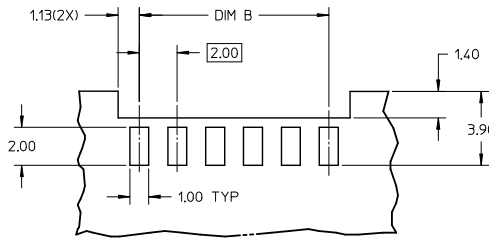
RECOMMENDED PCB PATTERN (PATTERN TYPICAL BOTH SIDES)
