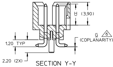
SECTION Y-Y
