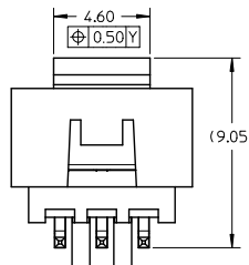
VIEW FOR HEADER WITH CAP
