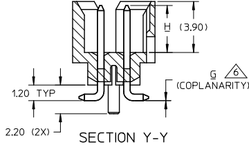
SECTION Y-Y
