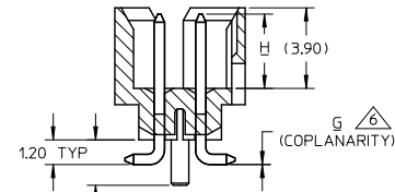
SECTION Y-Y
