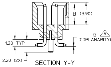
SECTION Y-Y
