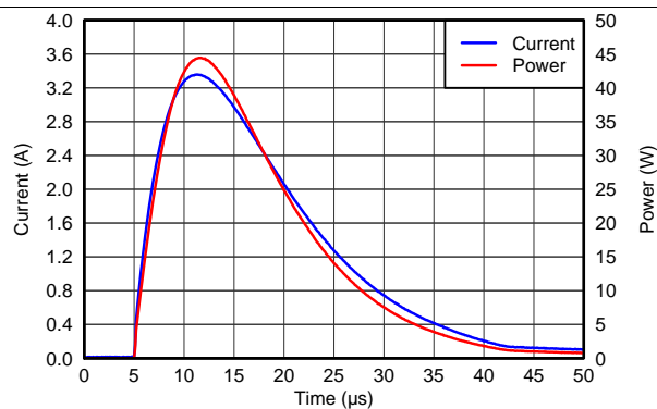
Figure 6. Surge Curves, Data to GND
