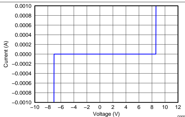
Figure 5. IV Curve
