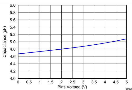
Figure 8. Capacitance
