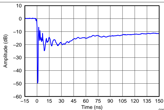
Figure 2. IEC 61000-4-2 Clamping Voltage, -8-kV Contact
