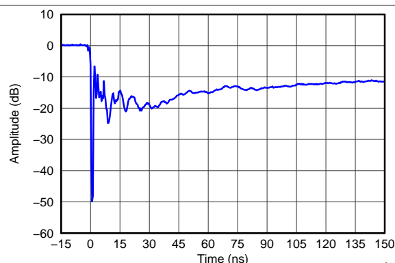
Figure 12. IEC 61000-4-2 Clamping Voltage, -8-kV Contact
