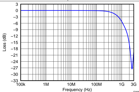
Figure 9. Insertion Loss
