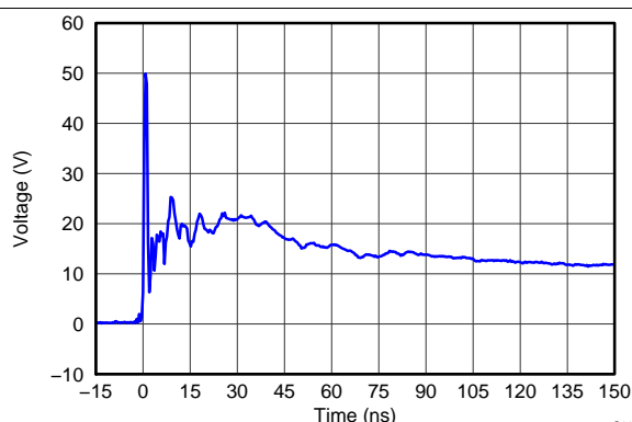
Figure 11. IEC 61000-4-2 Clamping Voltage, 8-kV Contact
