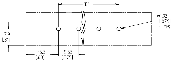
PTH PATTERN
