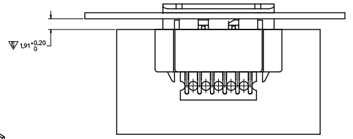
PANEL TO PCB STACK HEIGHT
