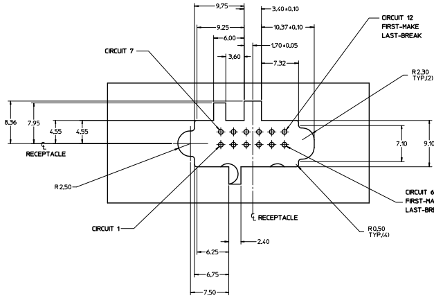
PANEL CUTOUT PANEL THICKNESS 1.20±0.12MM
