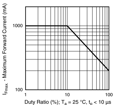
Fig. 5 - Forward Current vs. Duty Ratio
