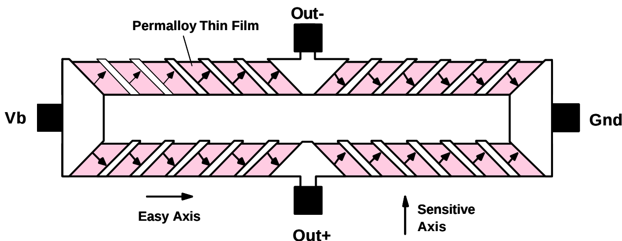
Figure 1 – Magneto-Resistive Wheatstone Bridge Elements
