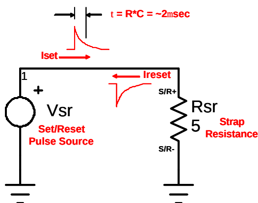
Figure 2 – A Simple Set/Reset Circuit
