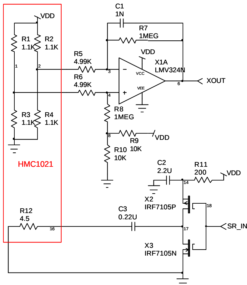
Figure 6 – Field Detector or Current Sensor
