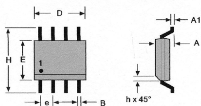
HMC1021S—8-Pin SOIC
