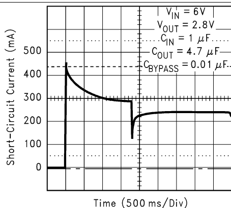
Figure 25. Short-Circuit Current
