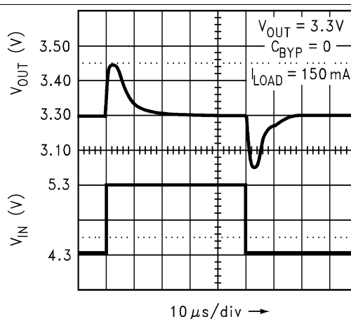
Figure 32. Line Transient Response
