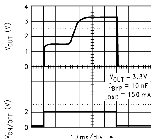
Figure 38. Turn-On Time
