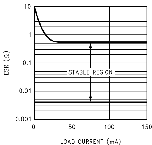
Figure 22. ESR Graph
