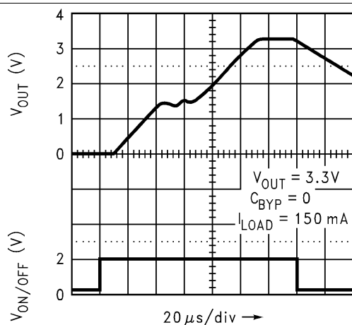
Figure 35. Turn-On Time
