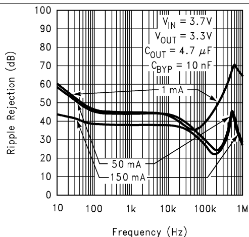
Figure 10. Ripple Rejection
