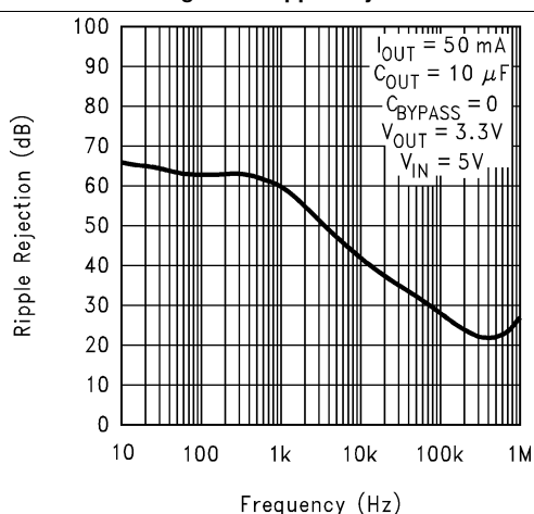
Figure 5. Ripple Rejection
