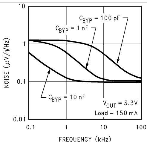
Figure 15. Output Noise Density
