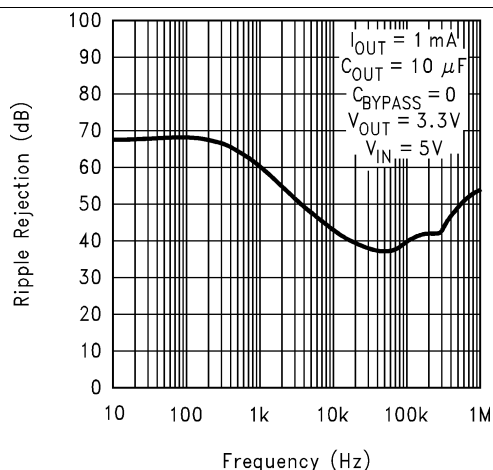
Figure 4. Ripple Rejection
