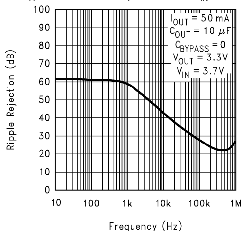
Figure 8. Ripple Rejection
