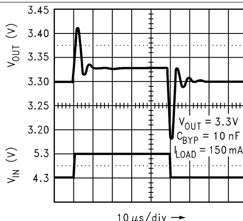
Figure 34. Line Transient Response
