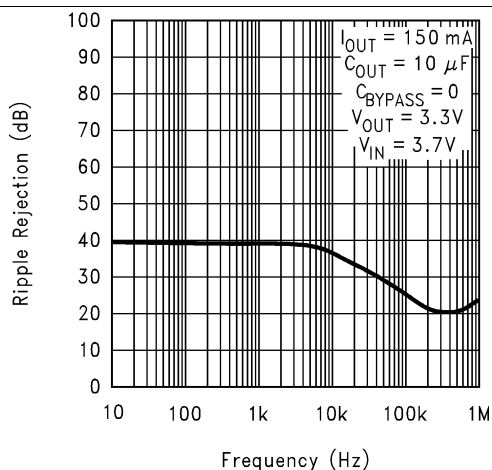
Figure 9. Ripple Rejection
