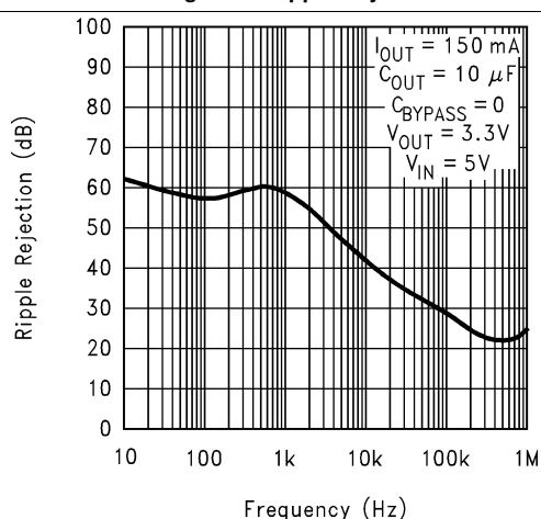
Figure 6. Ripple Rejection
