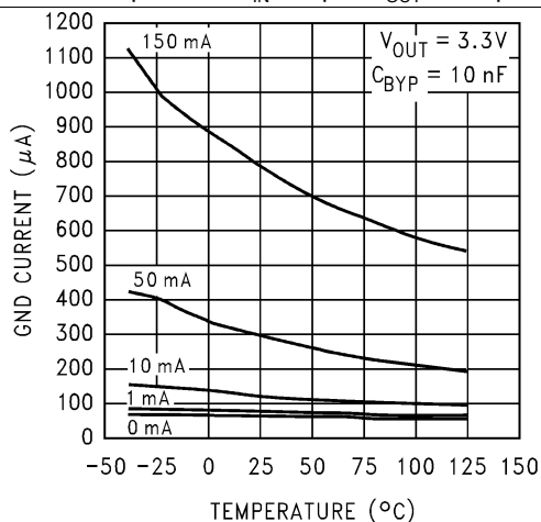
Figure 19. GND Pin Current vs Temperature
