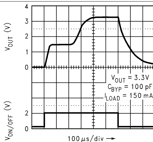
Figure 36. Turn-On Time
