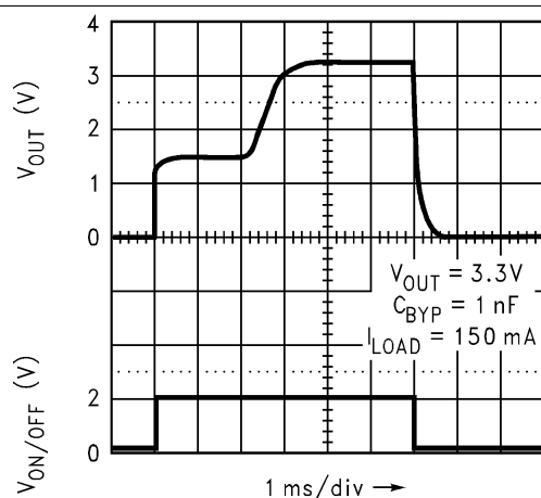
Figure 37. Turn-On Time
