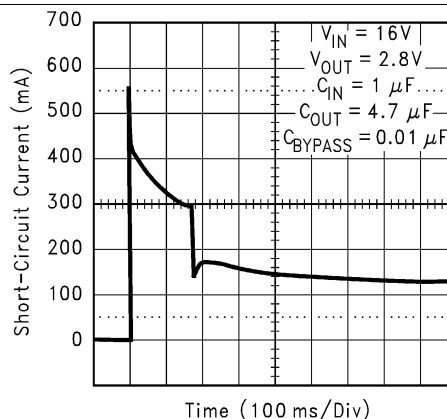
Figure 26. Short-Circuit Current
