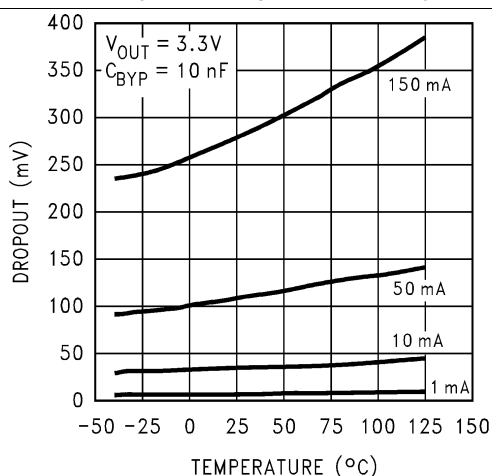
Figure 17. Dropout Voltage vs Temperature
