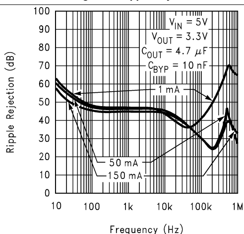
Figure 11. Ripple Rejection
