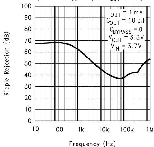
Figure 7. Ripple Rejection
