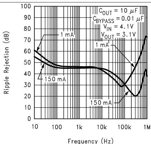
Figure 3. Ripple Rejection
