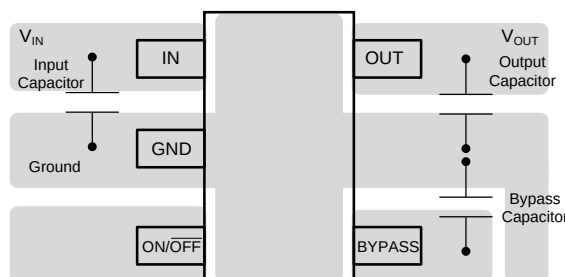
Figure 39. LP2985 SOT-23 Package Typical Layout
