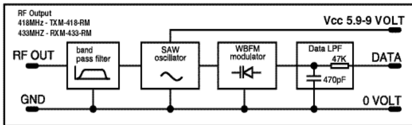
figure 1: LINX-TX block diagram
