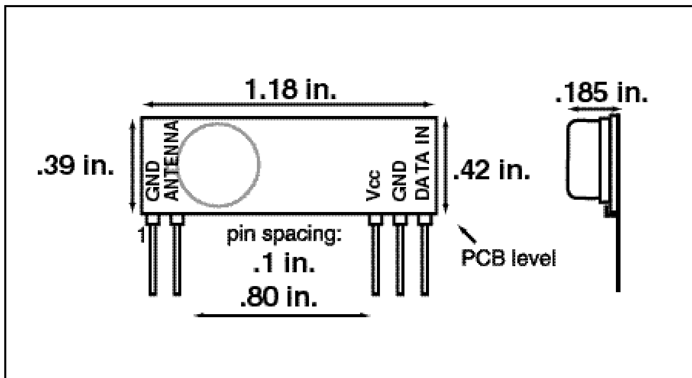
figure 2: Mechanical dimensions
