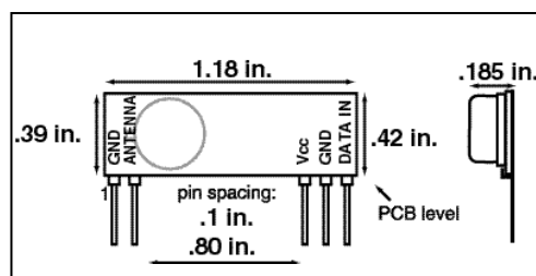
Physical Outline
