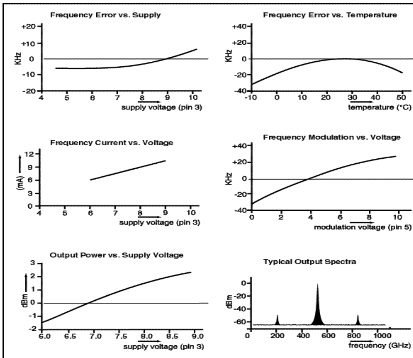
figure 4: Typical performance curves
