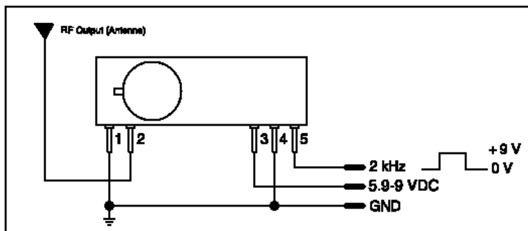
figure 3: LINX RM Series test circuit
