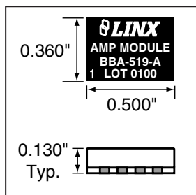
Figure 1: BBA Package Dimensions
