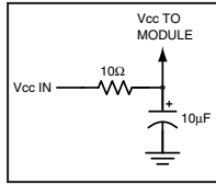
Figure 5: Supply Filter
