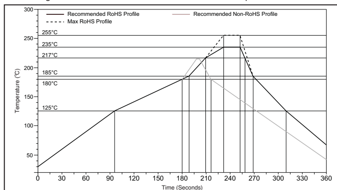
Figure 11: Maximum Reflow Profile
