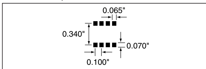
Figure 9: Recommended PCB Layout
