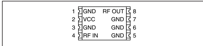
Figure 3: BBA Series Amplifier Pinout (Top View)
