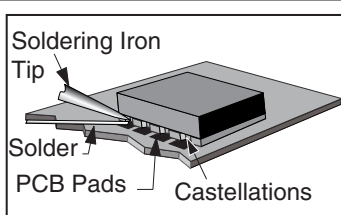
Figure 10: Soldering Technique
