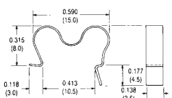
Speed Clip 330 SC 4 lb (17.8N) Nominal Force Installed
