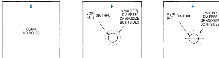
603 SERIES (EXTRUSION PROFILE 1284)
