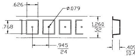
TAPE DETAILS
