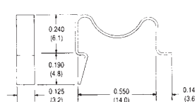
Speed Clip 285 SC 10 lb (44.5N) Nominal Force Installed
