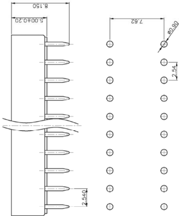
PCB LAYOUT
