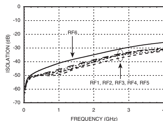
Isolation [1]
