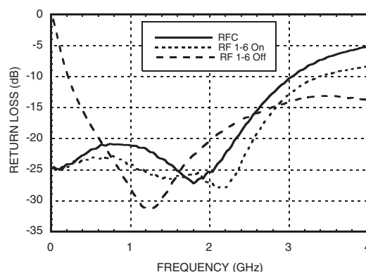
Return Loss [1]
