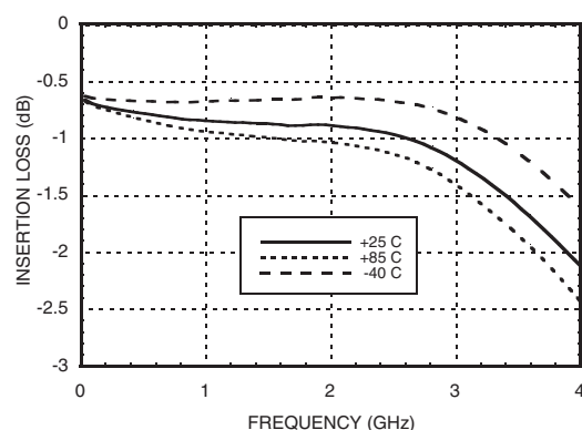
Insertion Loss [1]
