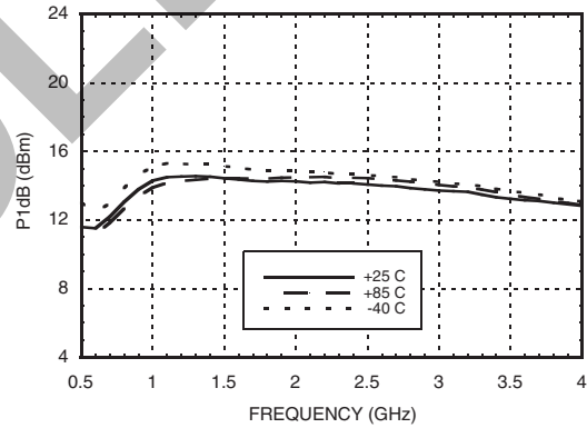
Output P1dB vs. Temperature @ Vdd = +3V
