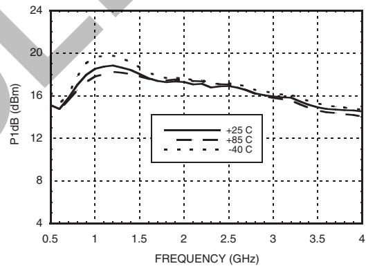
Output P1dB vs. Temperature @ Vdd = +5V
