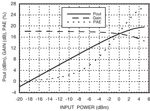
Power Compression @ 2.0 GHz, Vdd = +5V
