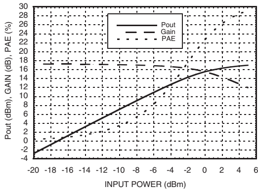
Power Compression @ 2.0 GHz, Vdd = +3V
