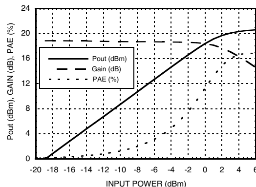
Power Compression @ 20 GHz
