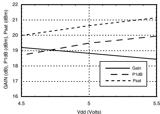
Gain, P1dB & PSAT vs. Supply Voltage @ 11 GHz
