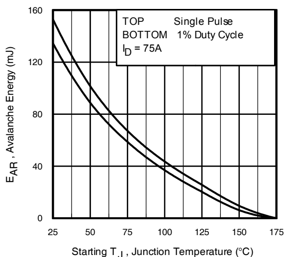
Fig 16. Maximum Avalanche Energy vs. Temperature
