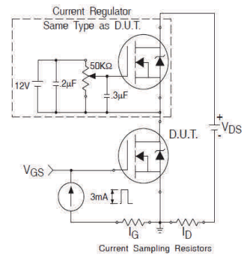
Fig 14b. Gate Charge Test Circuit
