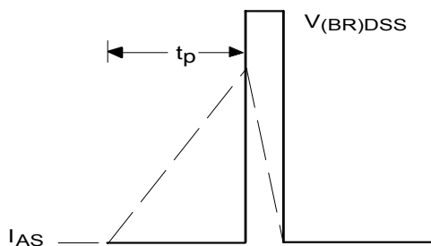
Fig 15b. Unclamped Inductive Waveforms
