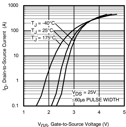
Fig 5. Transfer Characteristics
