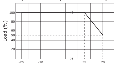
output power vs. ambient temperature (85~305 Vac; 120~430 Vdc)
