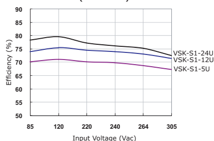
efficiency vs. input voltage (full load)
