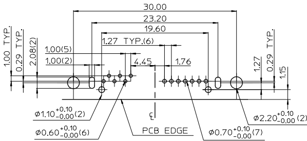
RECOMMENDED PC BOARD LAYOUT TOLERANCE:±0.05mm(TOP VIEW)
