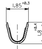
SECT. A-A
