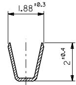
SECT. B-B
