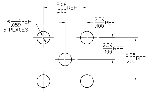
RECOMMENDED PCB PATTERN
