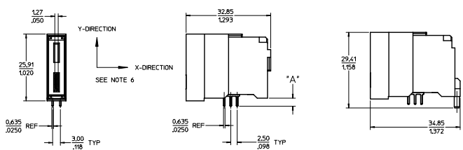
75561-5*** SHOWN (W/O PEG) SAME AS 75561-5*** EXCEPT AS SHOWN
