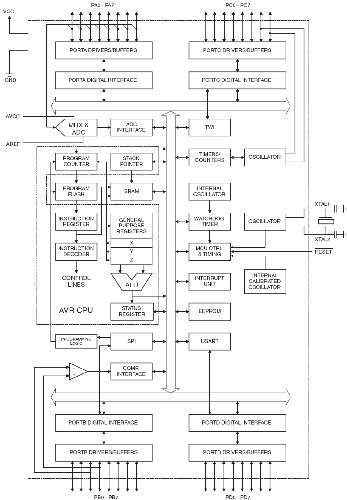
Figure 2. Block Diagram
