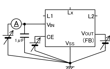
< Circuit No.④ >
