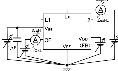
< Circuit No.⑦ >
