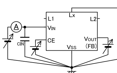
< Circuit No.⑩ >
