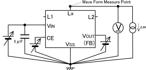
< Circuit No.⑧ >
