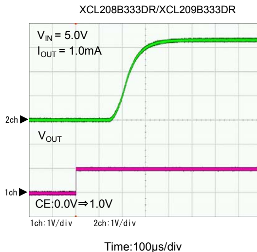
(12) Rise Wave Form
