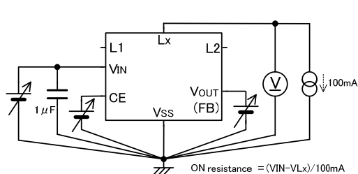
< Circuit No.⑥ >
