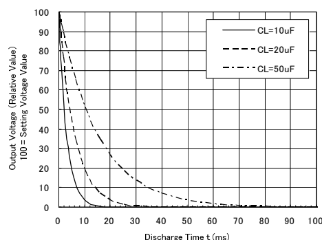
Output Voltage Discharge Characteristics R_{dischg} = 300\Omega (TYP)
