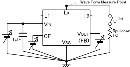
< Circuit No.⑨ >
