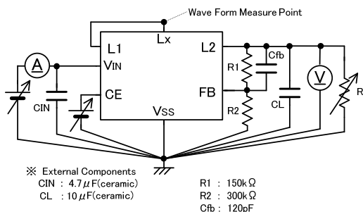
< Circuit No.③ >
