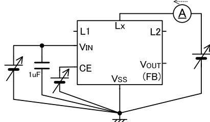
< Circuit No.⑩ >
