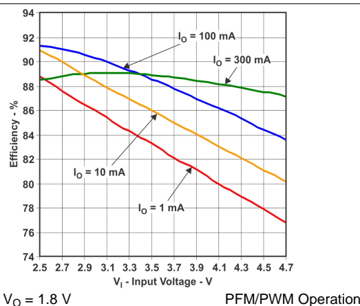
Figure 14. Efficiency vs. Input Voltage
