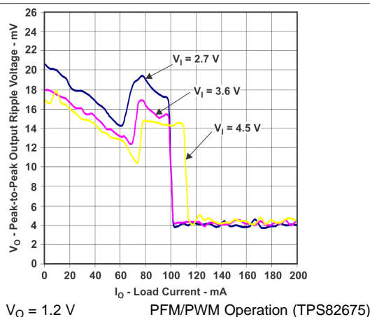
Figure 16. Peak-to-Peak Output Ripple Voltage vs. Load Current
