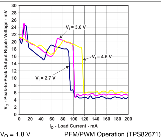
Figure 15. Peak-to-Peak Output Ripple Voltage vs. Load Current
