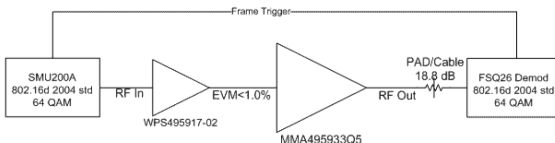
Figure 6 WiMax Test Setup
