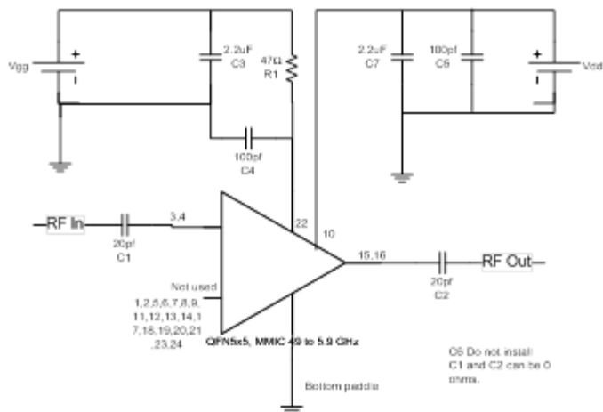
Figure 3 Evaluation Board Schematic
