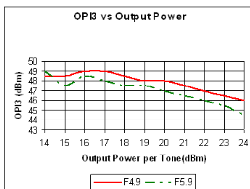
Figure 5 OIP3
