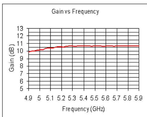
Figure 4 Gain Response
