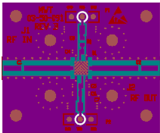
Figure 1 Evaluation Board
