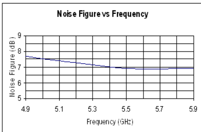
Figure 8 Noise Figure
