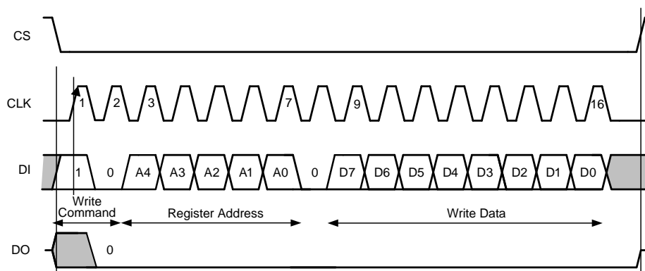
Figure 23. SPI Interface Write
