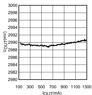
Figure 3. LDO V_{OUT} vs. I_{OUT}
