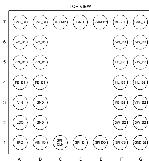
DSBGA 34 Top View
