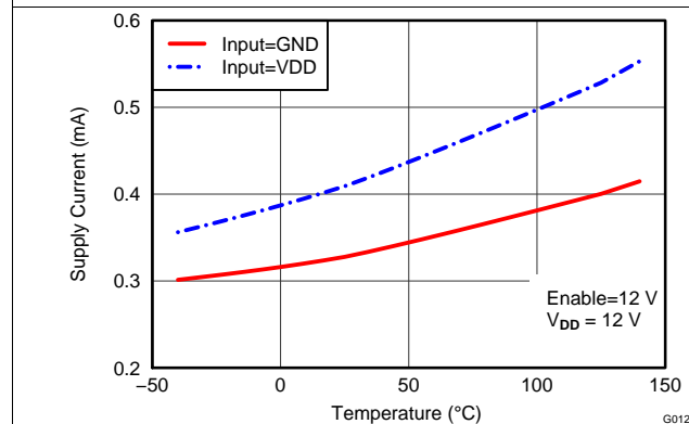
Figure 7. Supply Current vs Temperature (Outputs in DC ON/OFF Condition)
