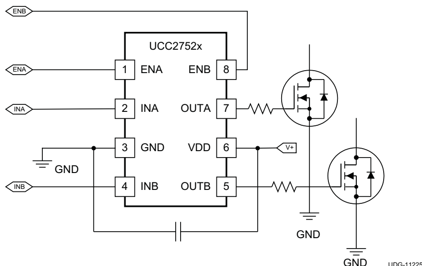
Figure 34. UCC2752x Typical Application Diagram (x = 3, 4, or 5)
