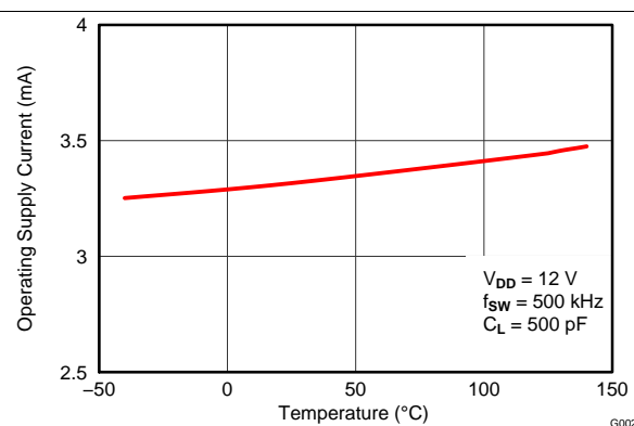
Figure 6. Operating Supply Current vs Temperature (Outputs Switching)
