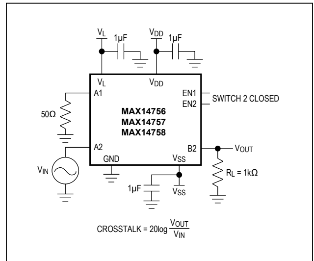
Figure 6. Crosstalk
