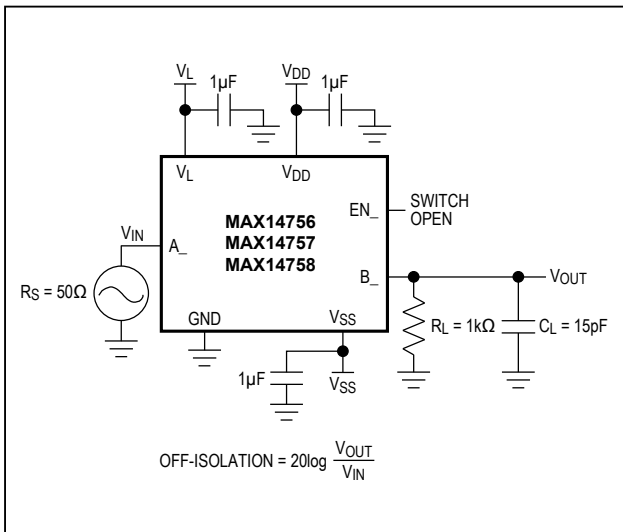
Figure 5. Off-Isolation
