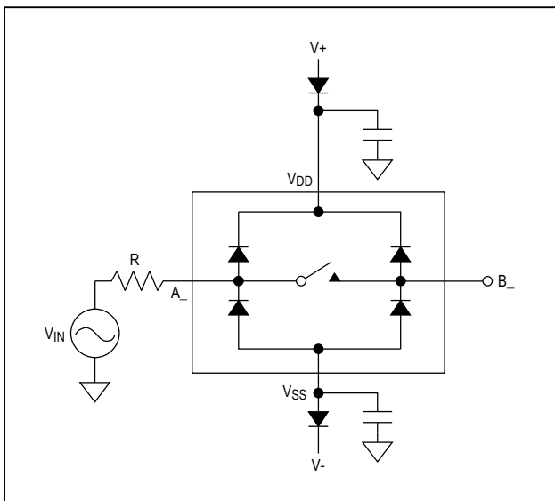
Figure 10. Beyond-the-Rail Application
