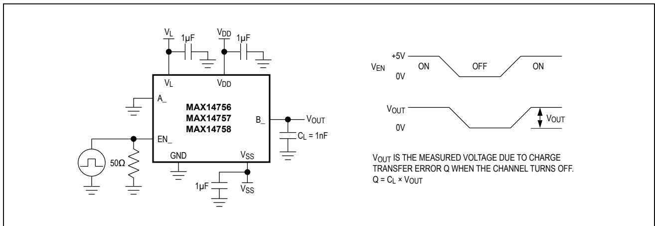
Figure 8. Charge Injection
