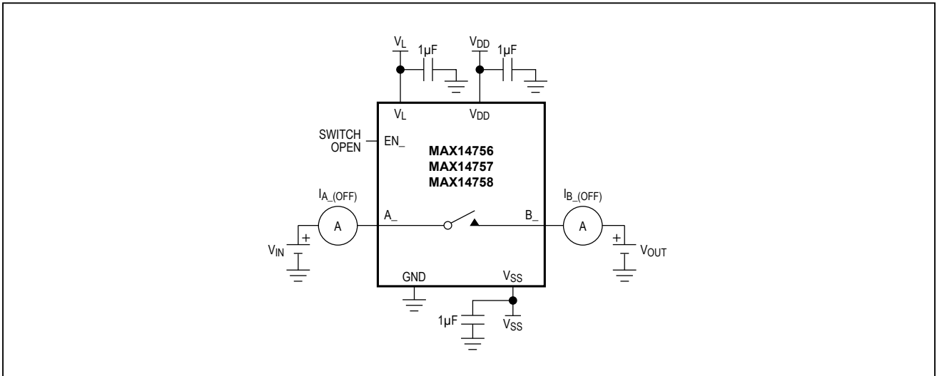
Figure 3. Off-Leakage Current
