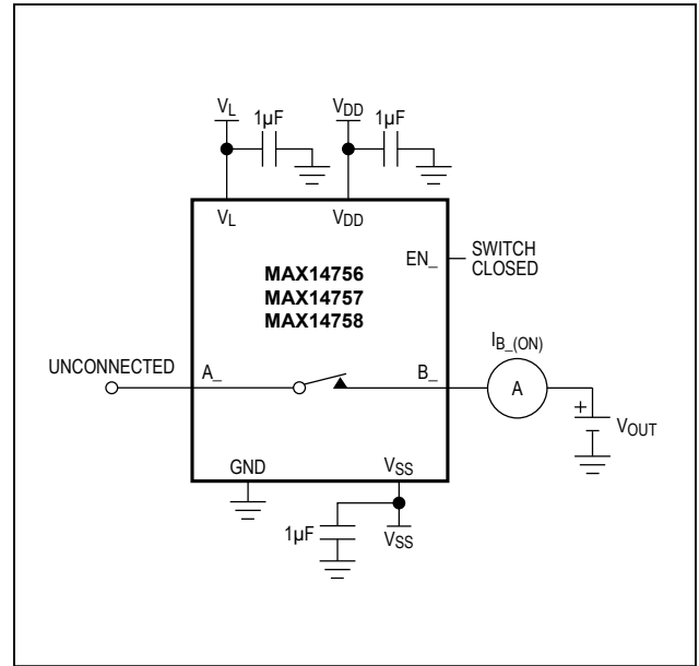
Figure 2. On-Leakage Current
