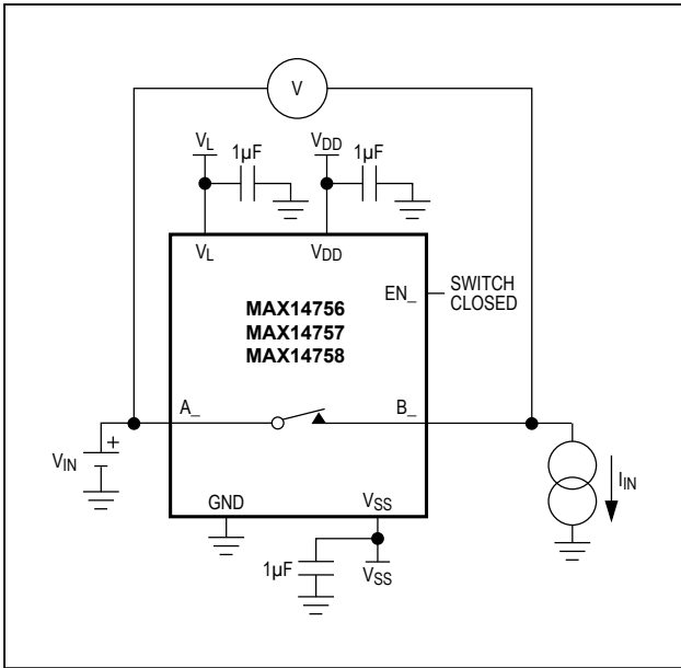
Figure 1. On-Resistance Measurement
