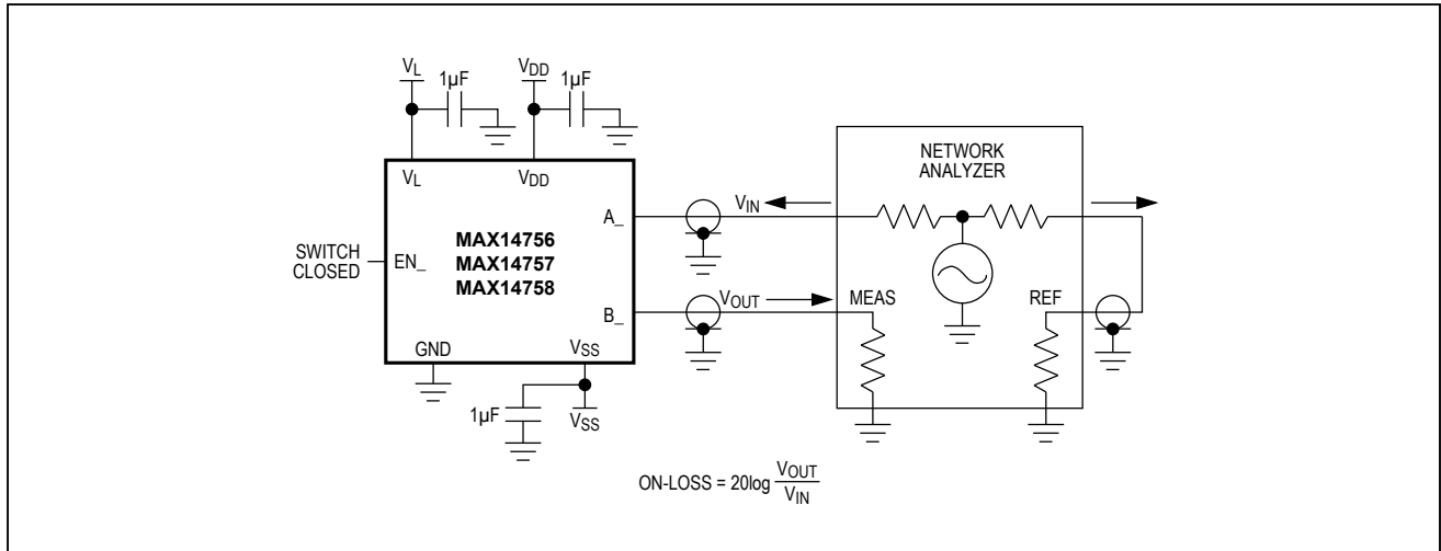
Figure 7. Frequency Response
