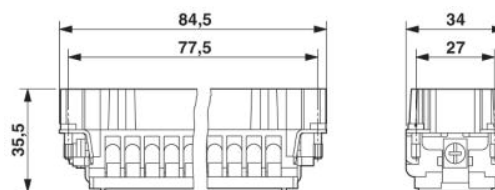
Male insert
