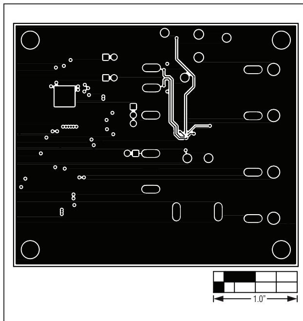
Figure 9. MAX97003 EV Kit PCB Layout—GND Layer 3
