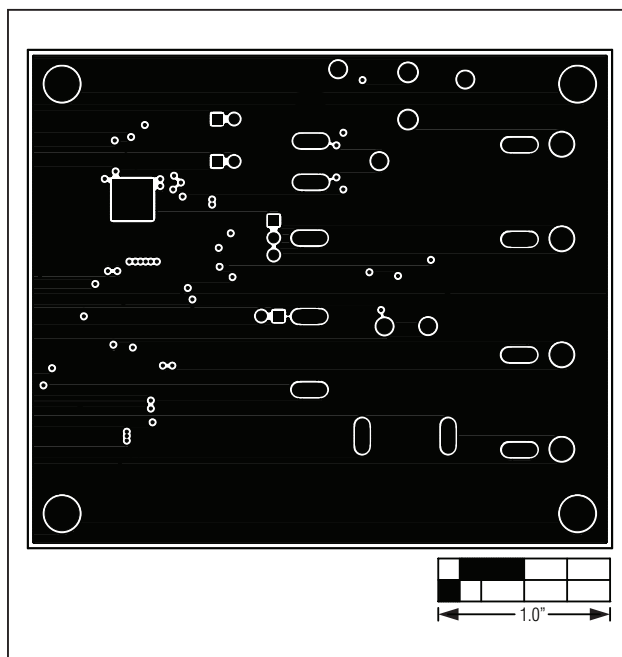
Figure 11. MAX97003 EV Kit PCB Layout—GND Layer 5
