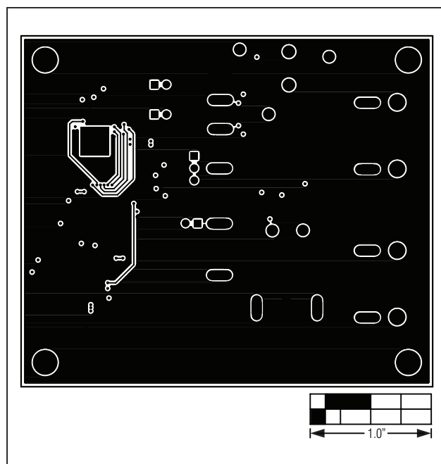
Figure 12. MAX97003 EV Kit PCB Layout—Solder Side
