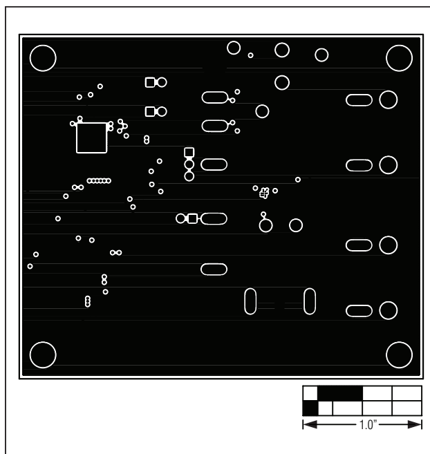
Figure 8. MAX97003 EV Kit PCB Layout—GND Layer 2
