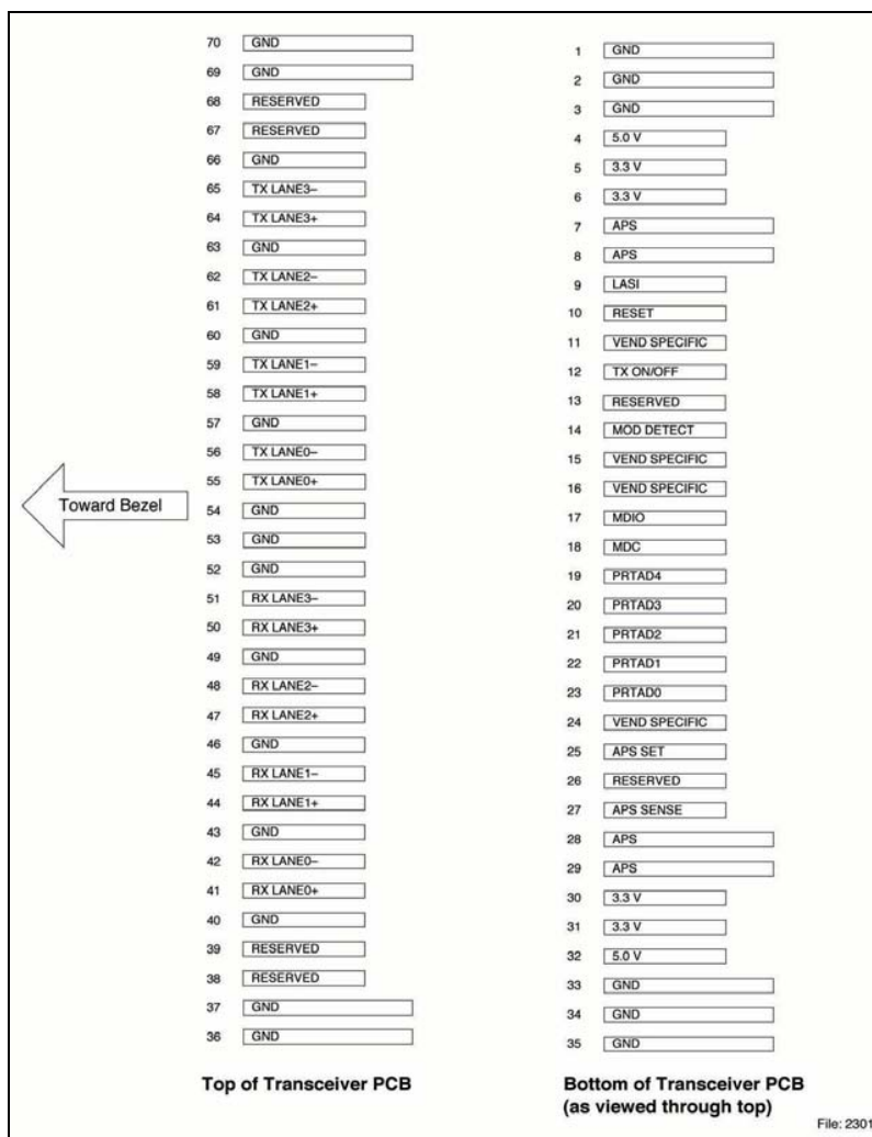
Figure 1- X2 Transponder Electrical Pad Layout
