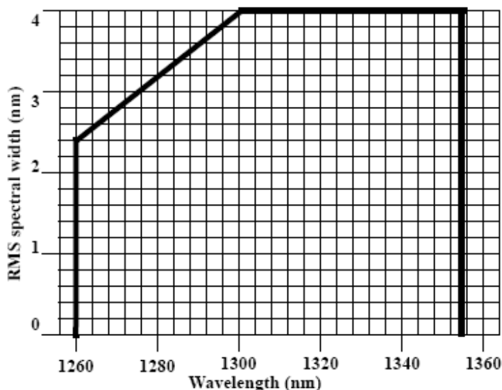
Figure 2-Transmitter Maximum RMS Spectral Width
