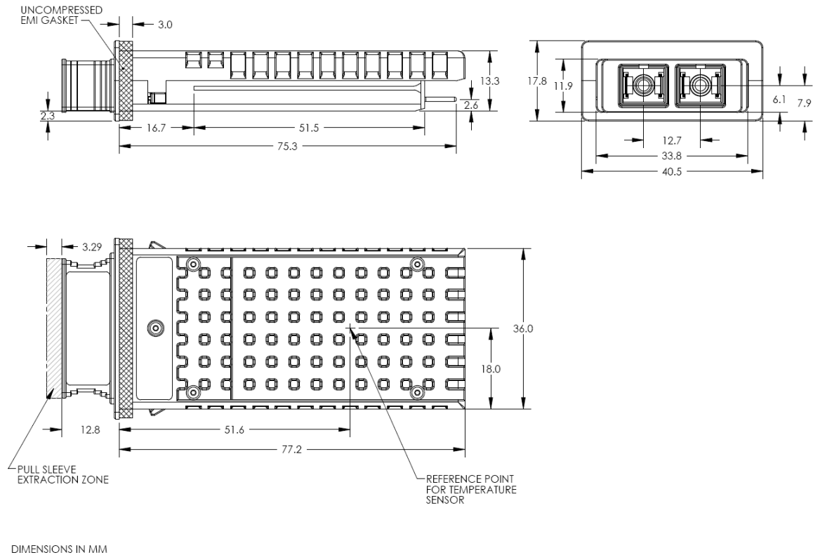
Figure 3-X2 Mechanical Dimensions
