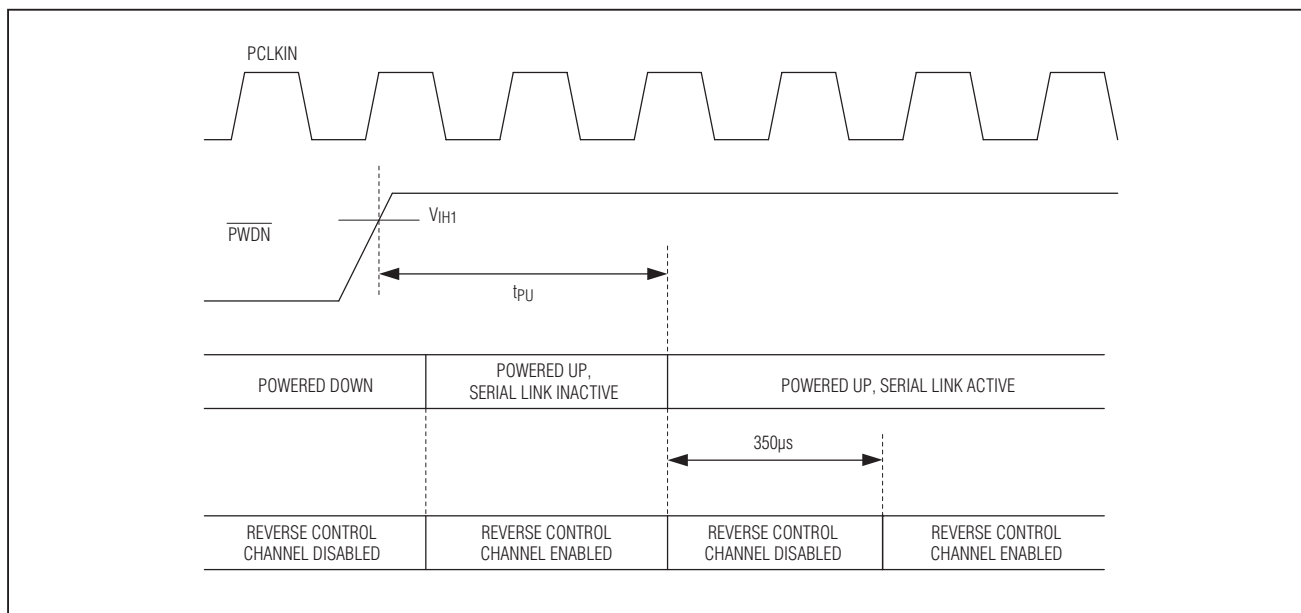
Figure 12. Power-Up Delay
