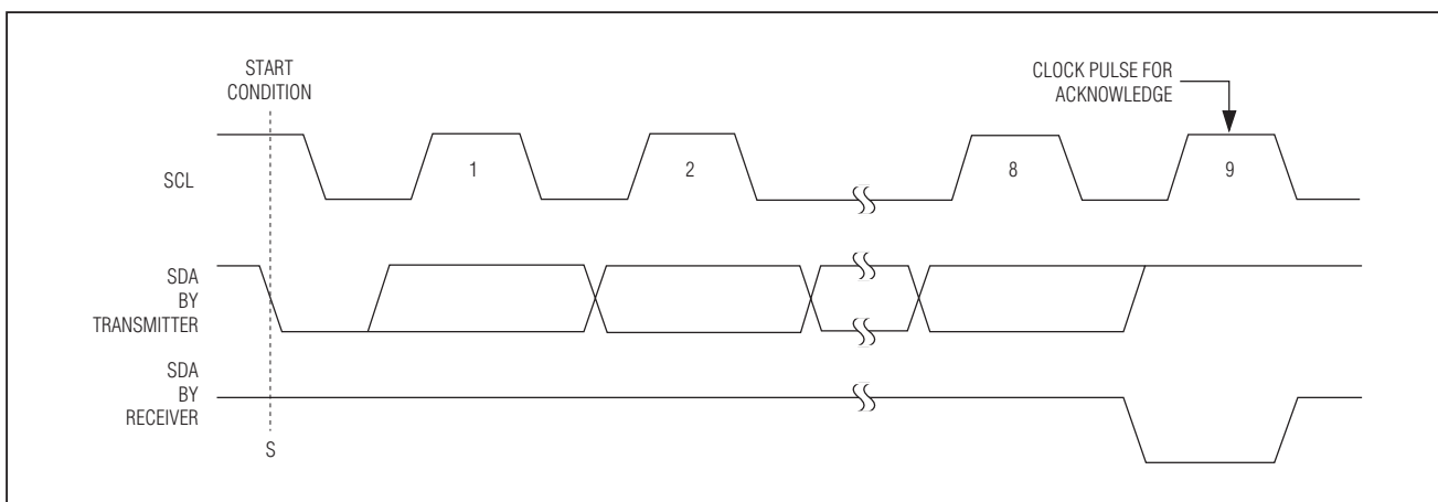
Figure 26. Acknowledge
