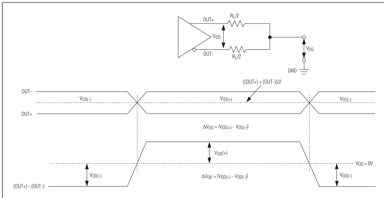
Figure 1. Serial-Output Parameters
