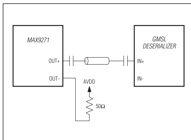
Figure 32. Coax-Mode Connection Diagram
