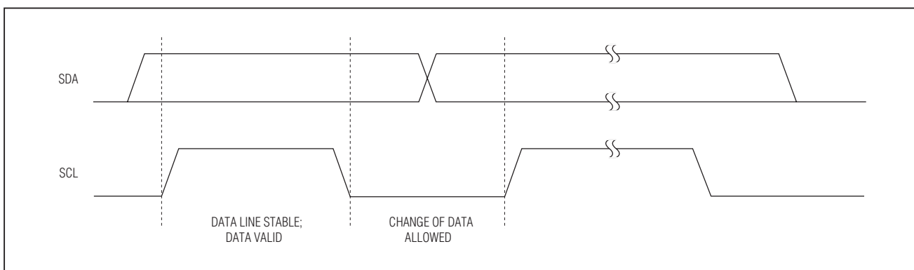
Figure 25. Bit Transfer
