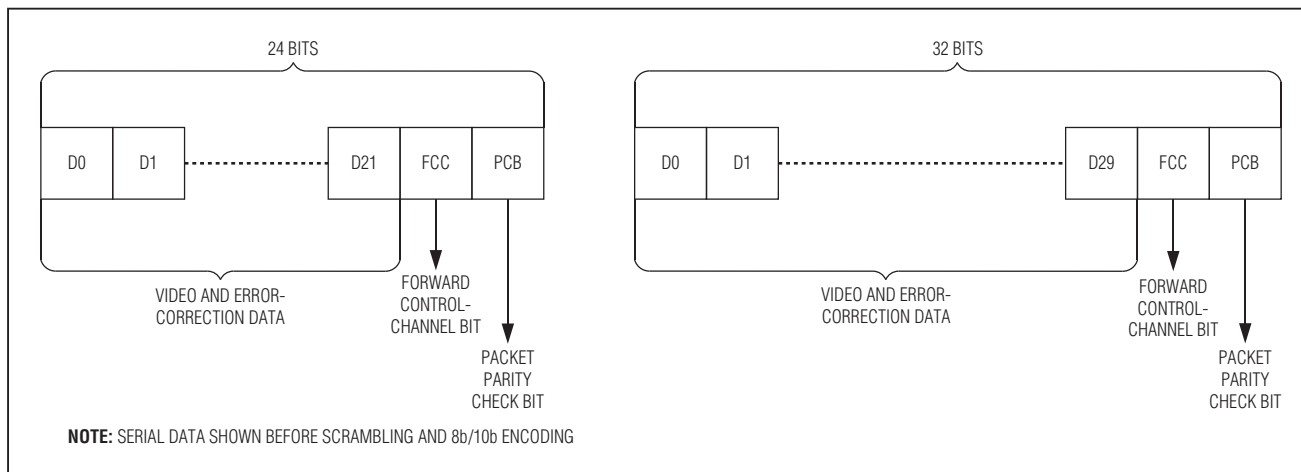
Figure 17. Serial-Data Format
