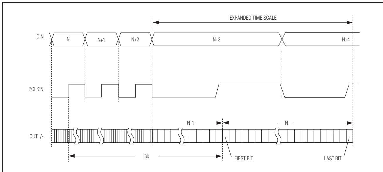
Figure 10. Serializer Delay
