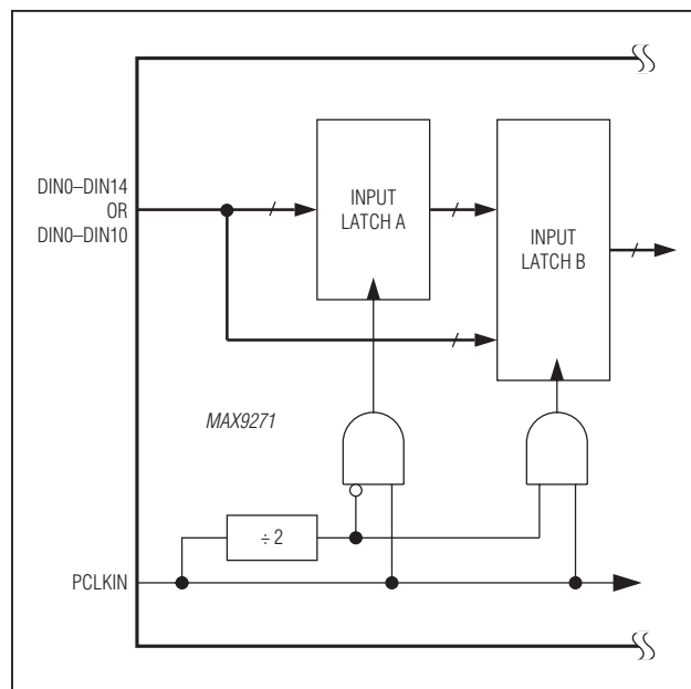
Figure 15. Double-Input Function Block
