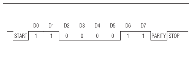
Figure 21. ACK Byte (0xC3)
