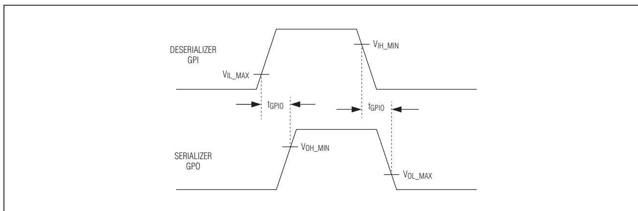
Figure 9. GPI-to-GPO Delay
