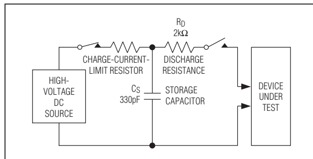
Figure 36. ISO 10605 Contact Discharge ESD Test Circuit
