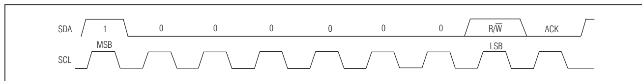
Figure 27. Slave Address
