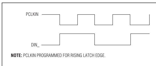
Figure 4. Worst-Case Pattern Input
