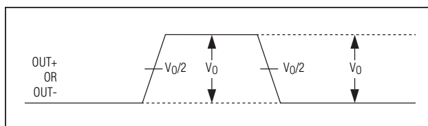
Figure 3. Single-Ended Output Template
