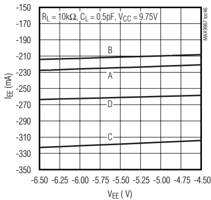
SUPPLY CURRENT, I EE vs. V EE
