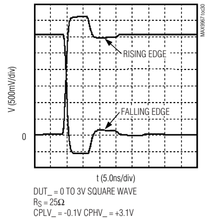
CLAMP RESPONSE
