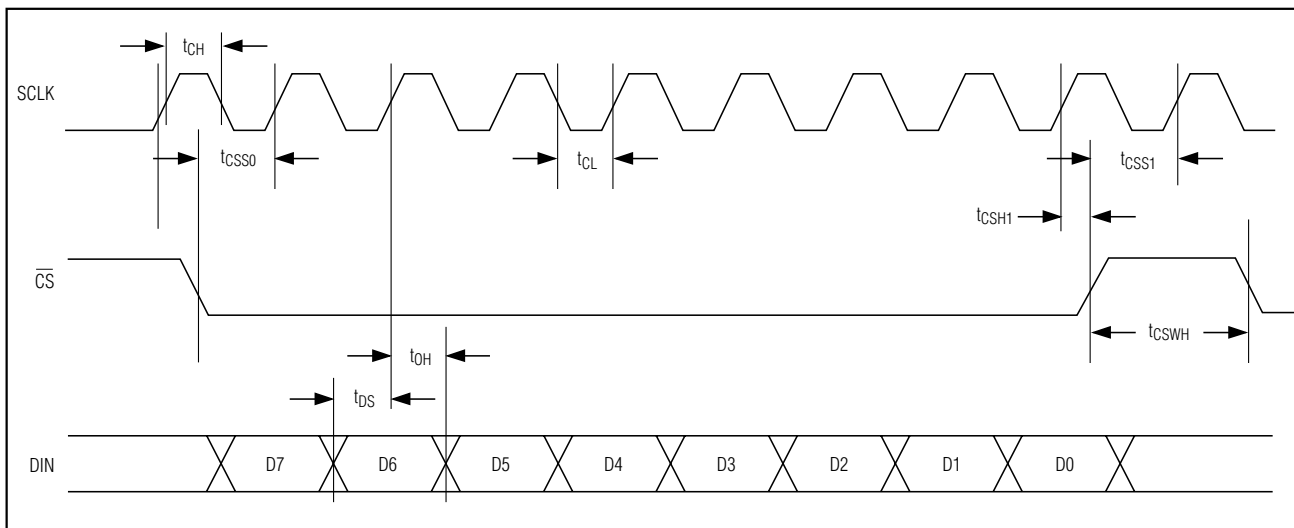
Figure 6. Serial-Interface Timing
