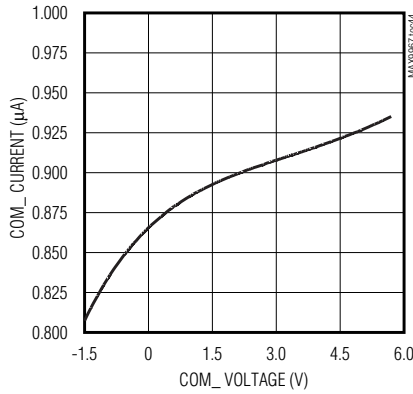
INPUT CURRENTS vs. INPUT VOLTAGE, COM_
