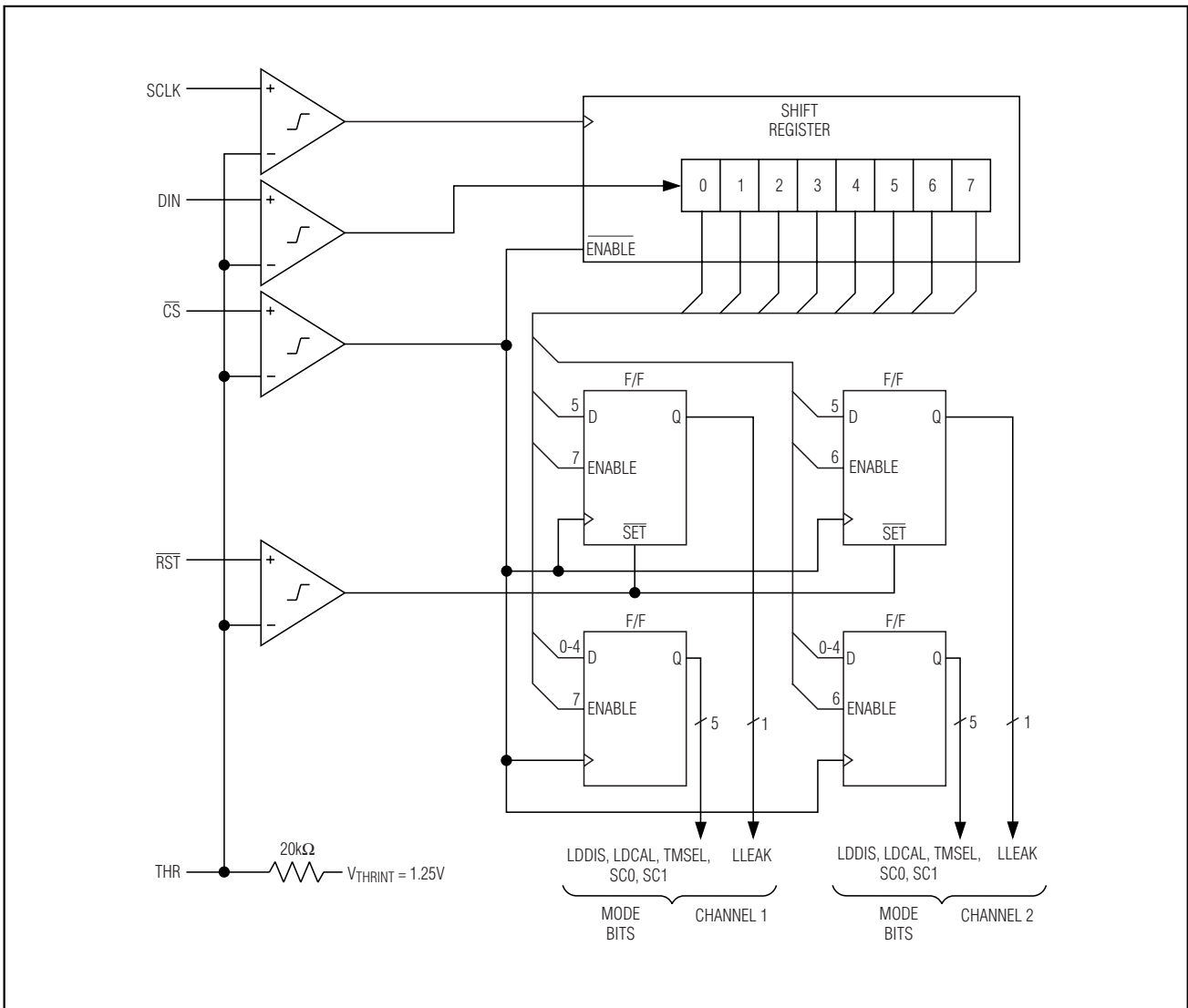
Figure 5. Serial Interface
