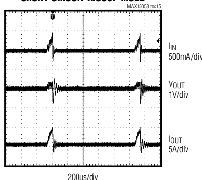
SHORT-CIRCUIT HICCUP MODE
