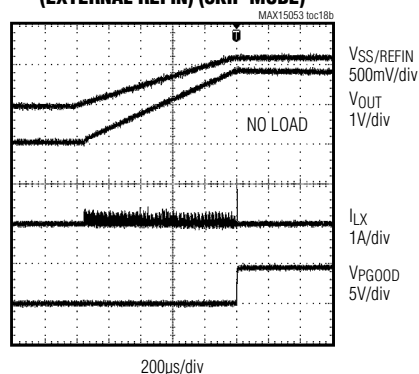
SOFT-START WAVEFORMS (EXTERNAL REFIN) (SKIP MODE)
