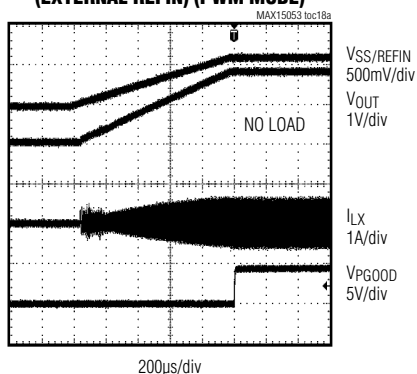
SOFT-START WAVEFORMS (EXTERNAL REFIN) (PWM MODE)
