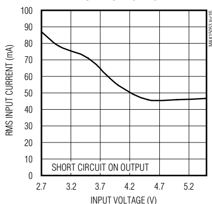
RMS INPUT CURRENT vs. INPUT VOLTAGE
