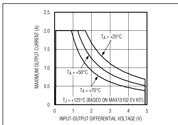
Figure 1. Maximum Output Current Curves
