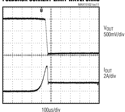
FOLDBACK CURRENT-LIMIT WAVEFORMS
