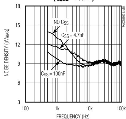
NOISE DENSITY ( I_{LOAD} = 100mA )
