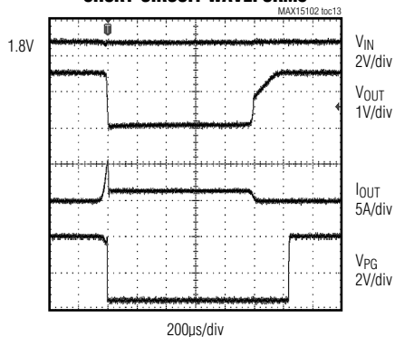
SHORT-CIRCUIT WAVEFORMS
