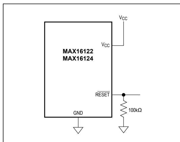
Figure 2. Ensuring \overline{\text{RESET}} Output to V_{CC} = 0V
