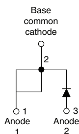
TO-247AC modified
